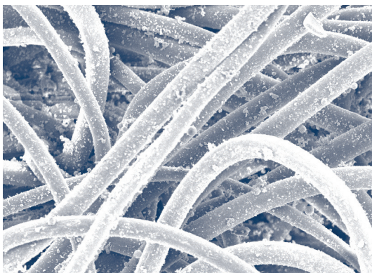
Needed Polyester Bag Clean Air Side (300x)
